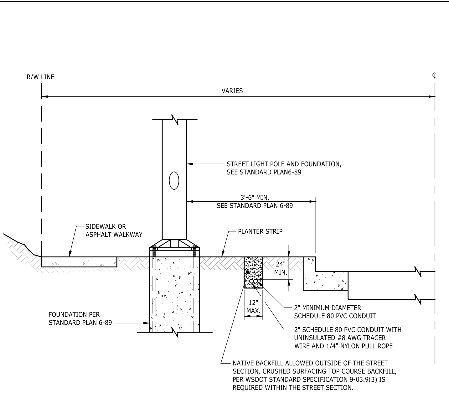
TYPICAL HALF ROADWAY SECTION
