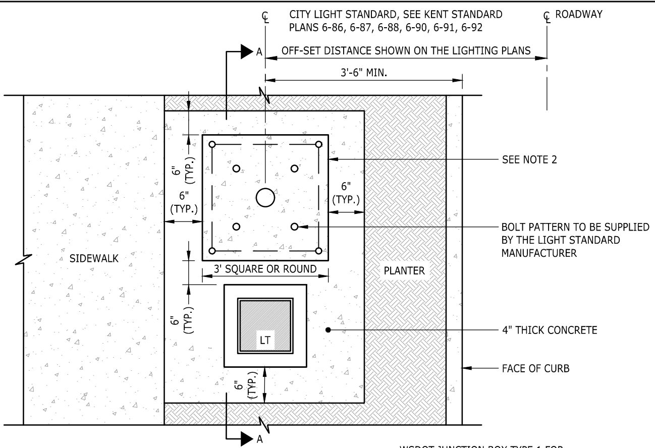
PLAN VIEW
