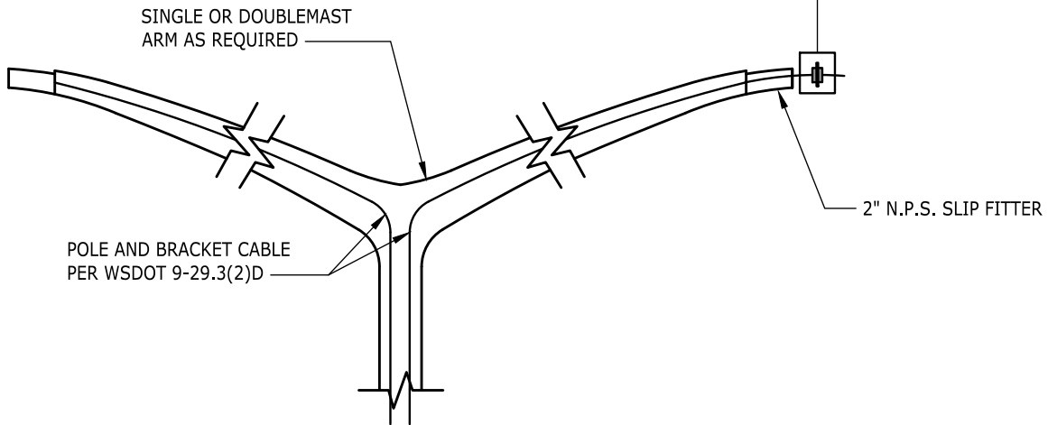
MAST ARM WIRING DETAIL
