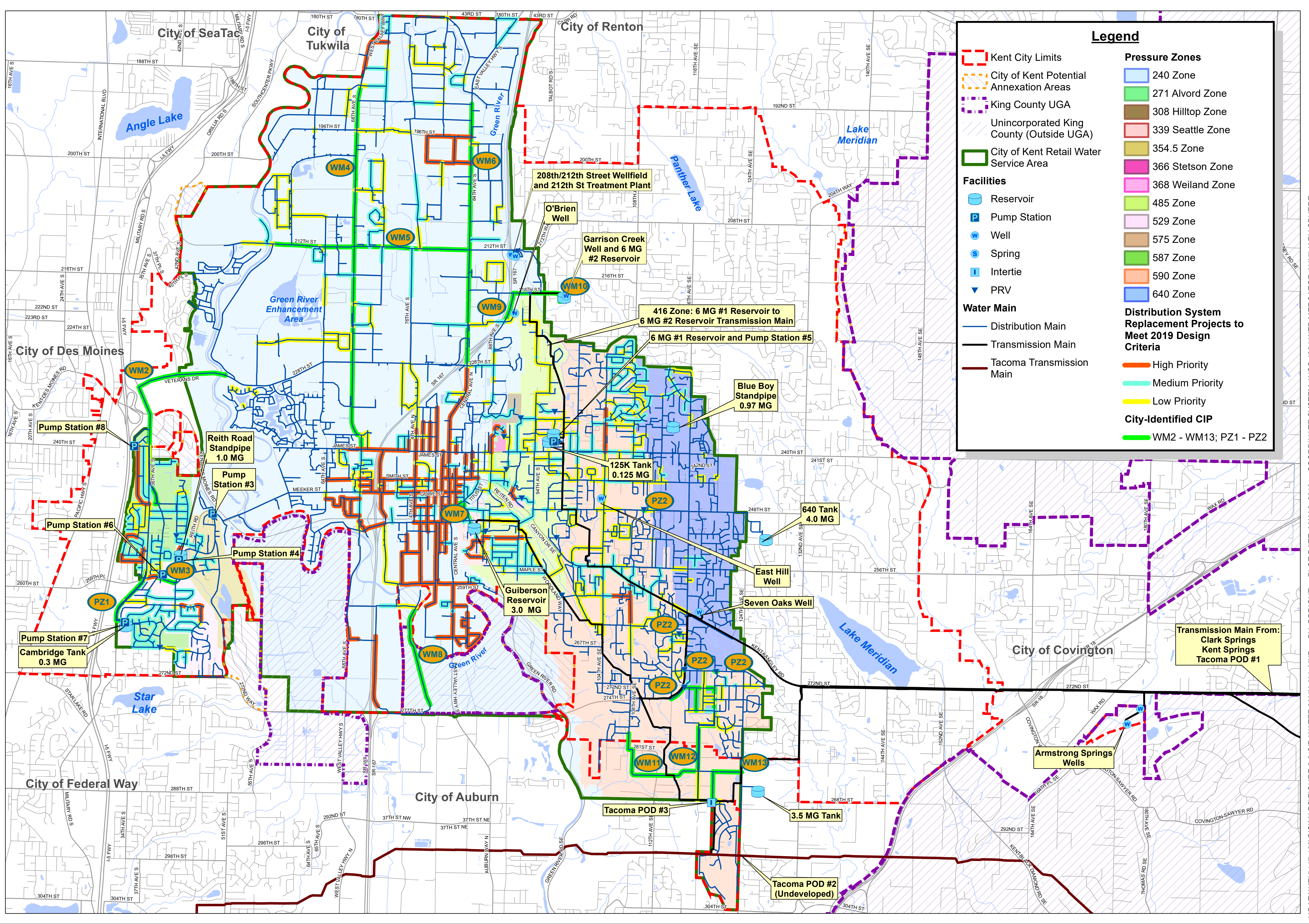
Figure 9-9 Water Main Projects System-wide City of Kent 2019 Water System Plan
