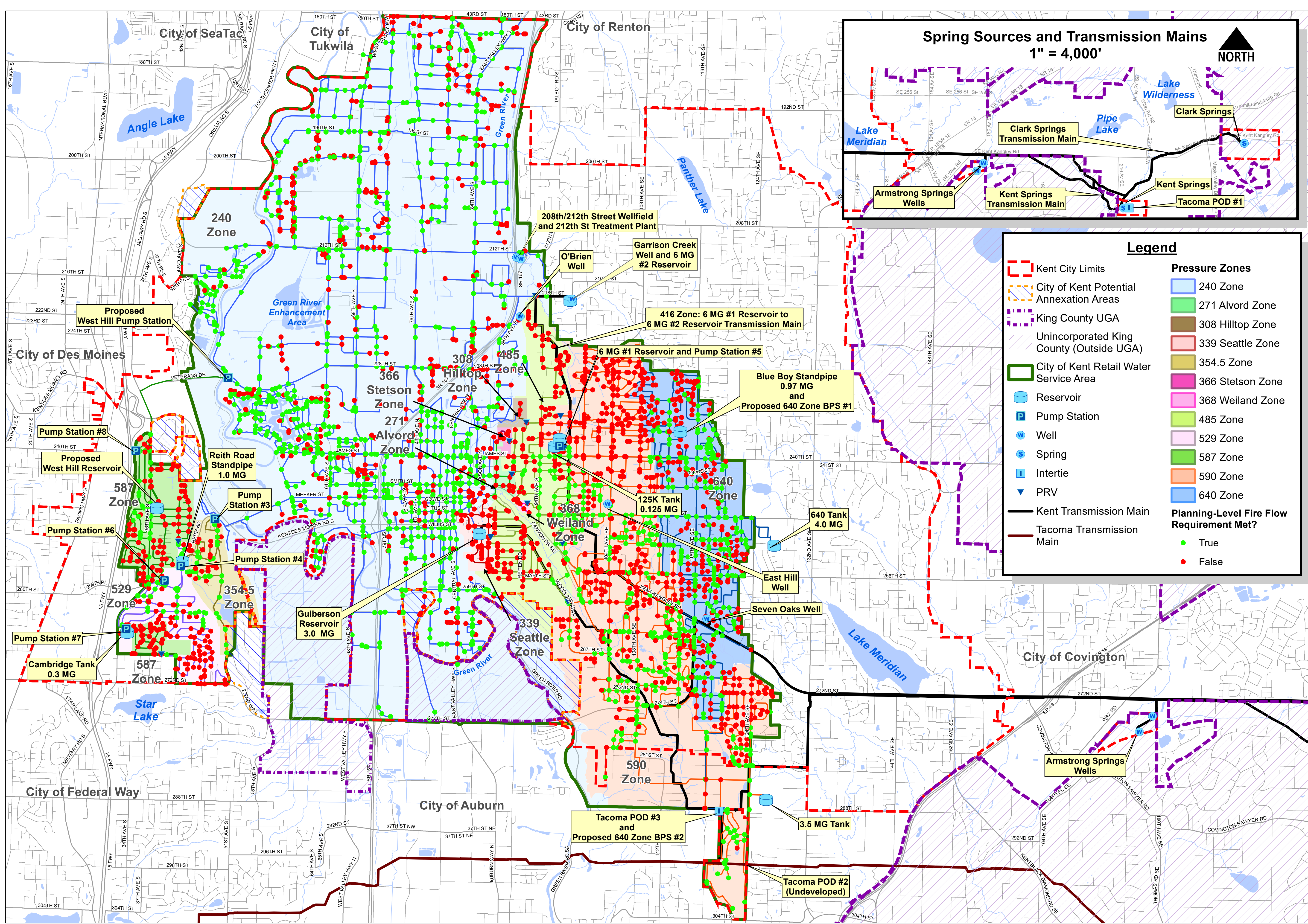
Figure 7-4 Projected 20-yr Junctions Exceeding FF Req't w/ City-Funded & High Priority Imprvmts. City of Kent 2019 Water System Plan
