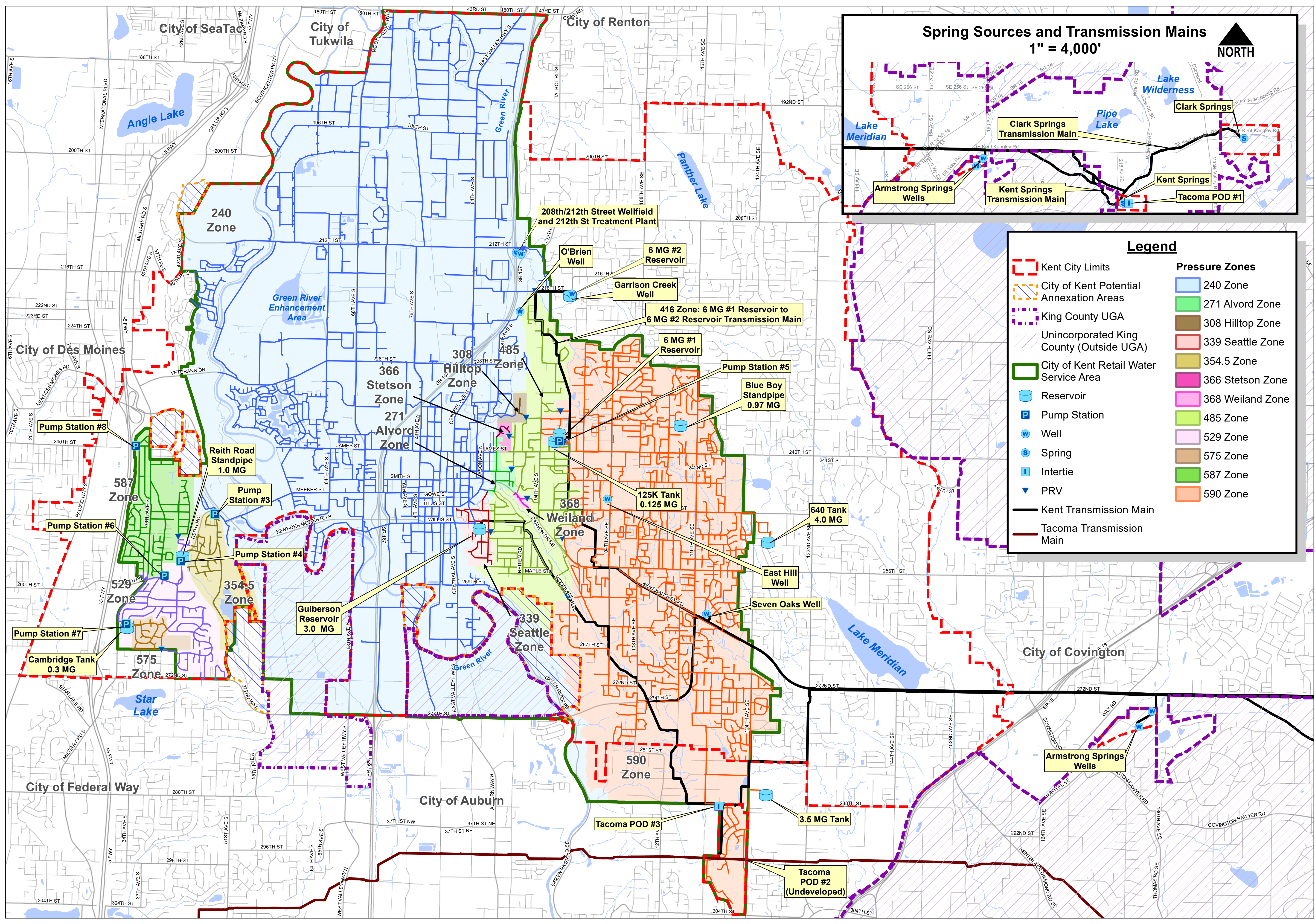
Figure 2-1 Existing Water System City of Kent 2018 Water System Plan
