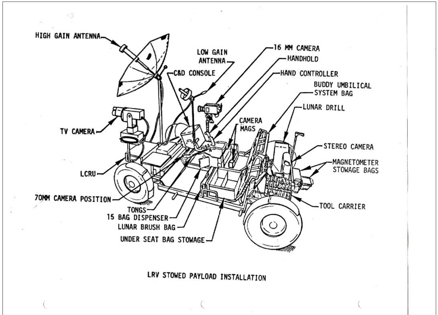
Figure 28: NASA-Marshall Space Flight Center. News release of LRV Line Drawing: LRV Stowed Payload Installation. Photo 0-10844. Release date March 1, 1971. The Boeing Company, Corporate Archives. Bellevue, WA.
